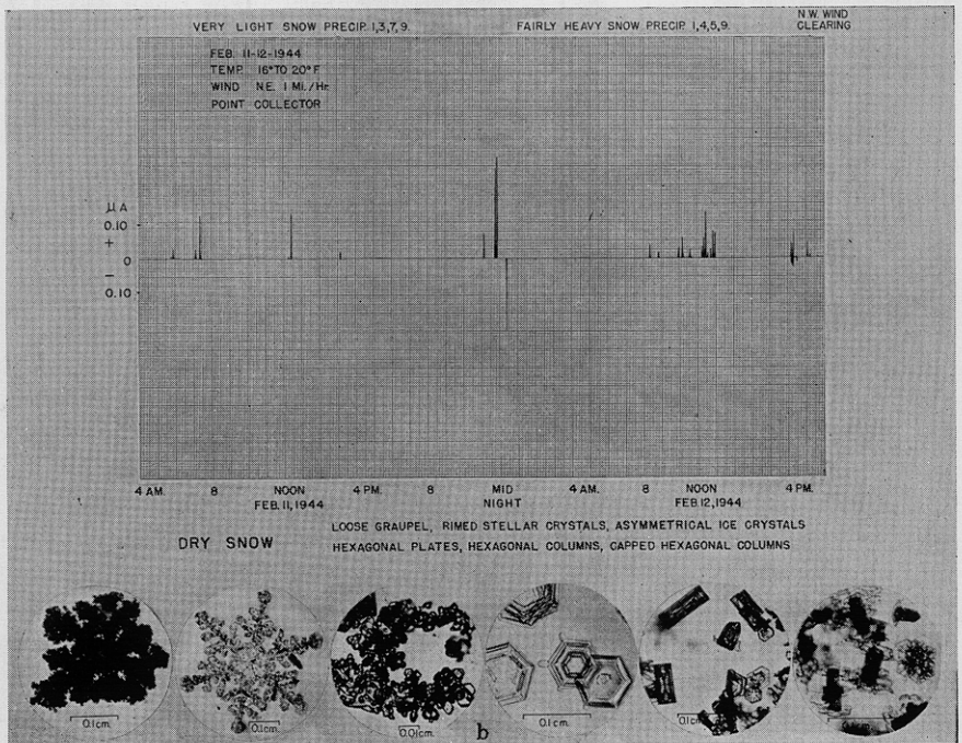
FIG. 2. Typical atmospheric electricity from positive current and cross current snow-storms.
